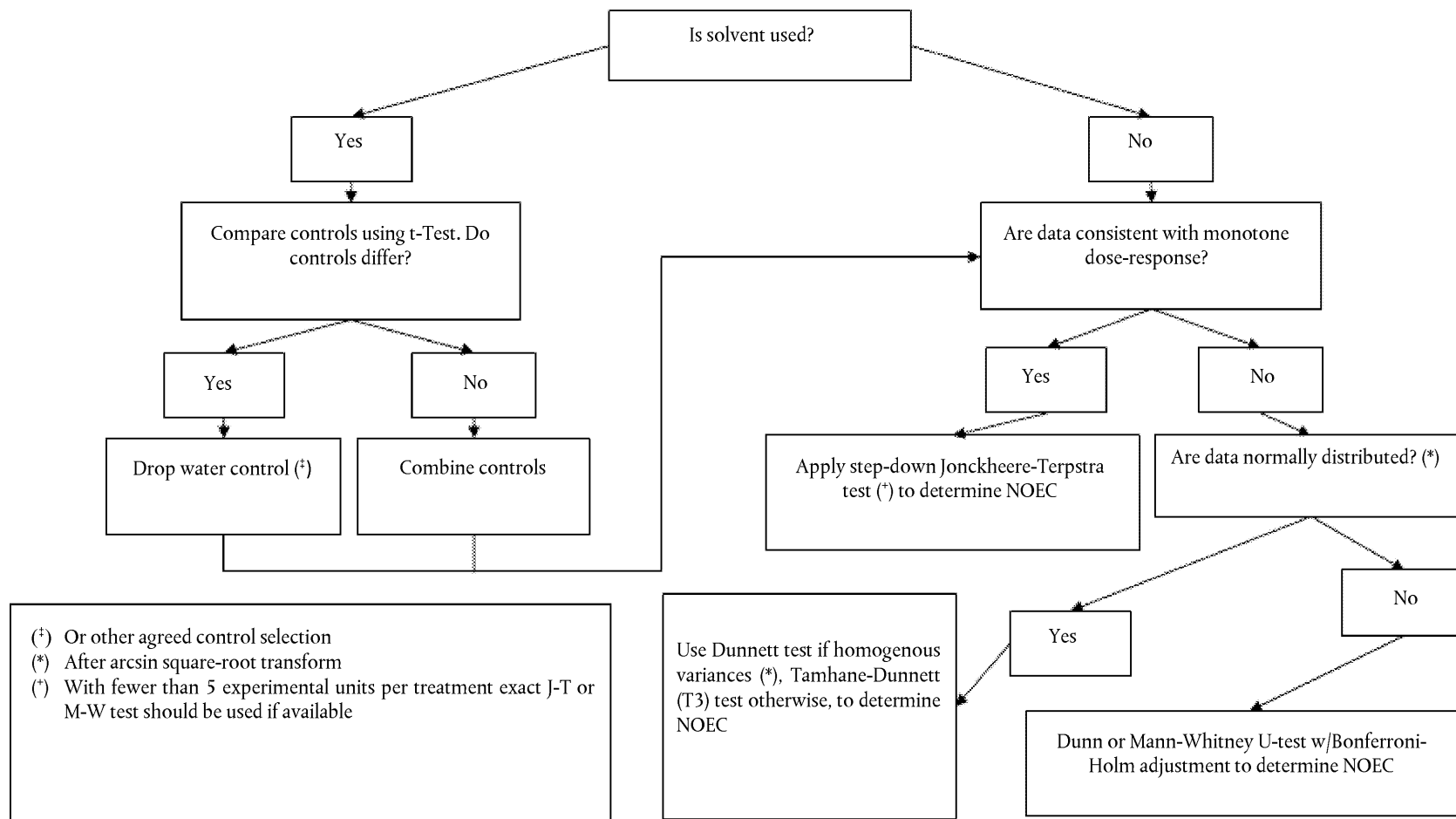
Statistical Flow Chart for sex ratio analysis
