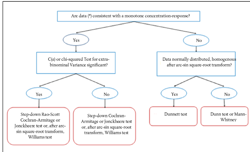
NOEC Flow Chart for Egg Hatch and Larval Mortality
