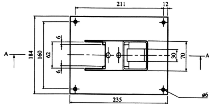
Figure 2 Support stand
