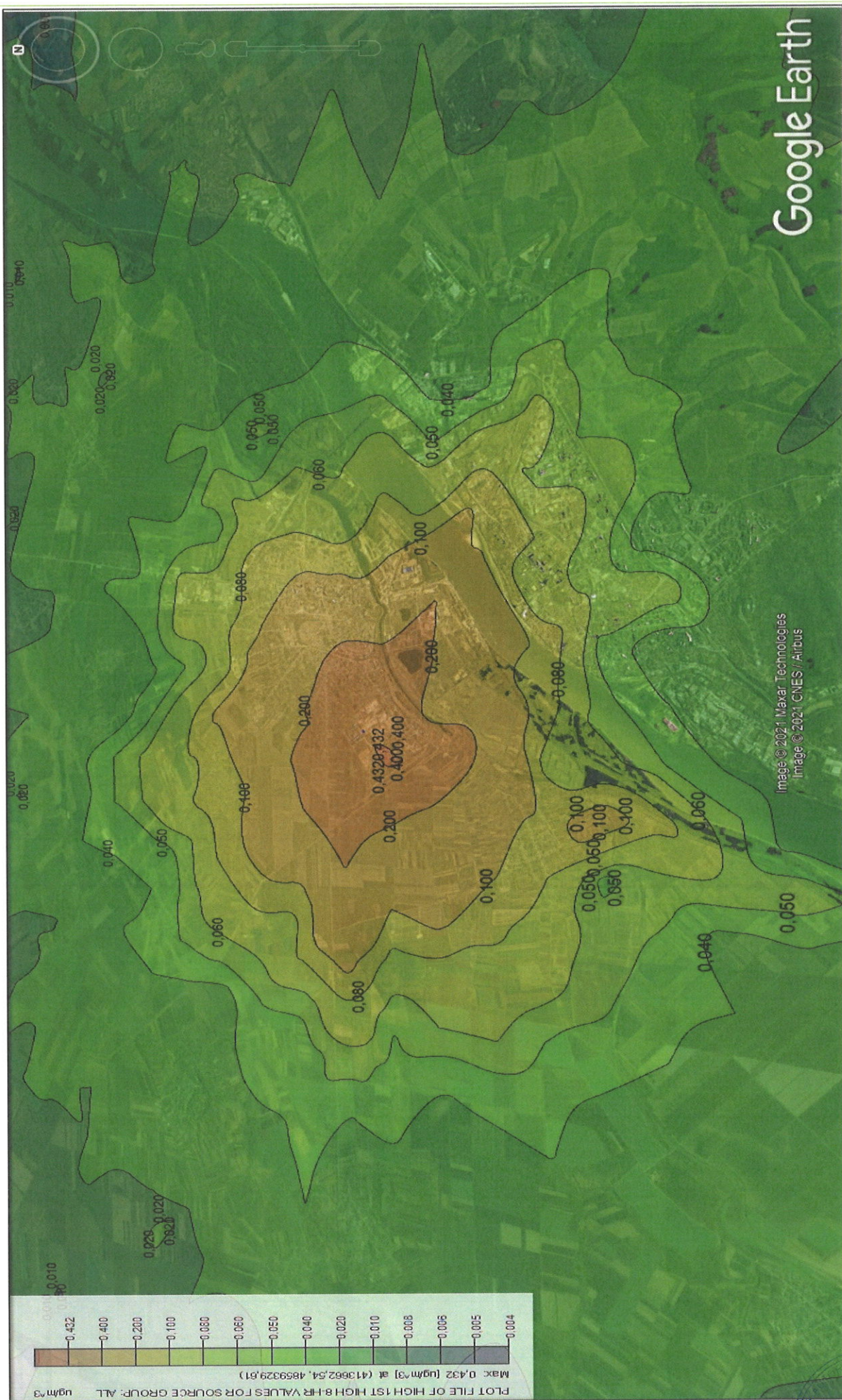
Figure 47 - CO dispersion modelling - averaging period 8 h (detail)
