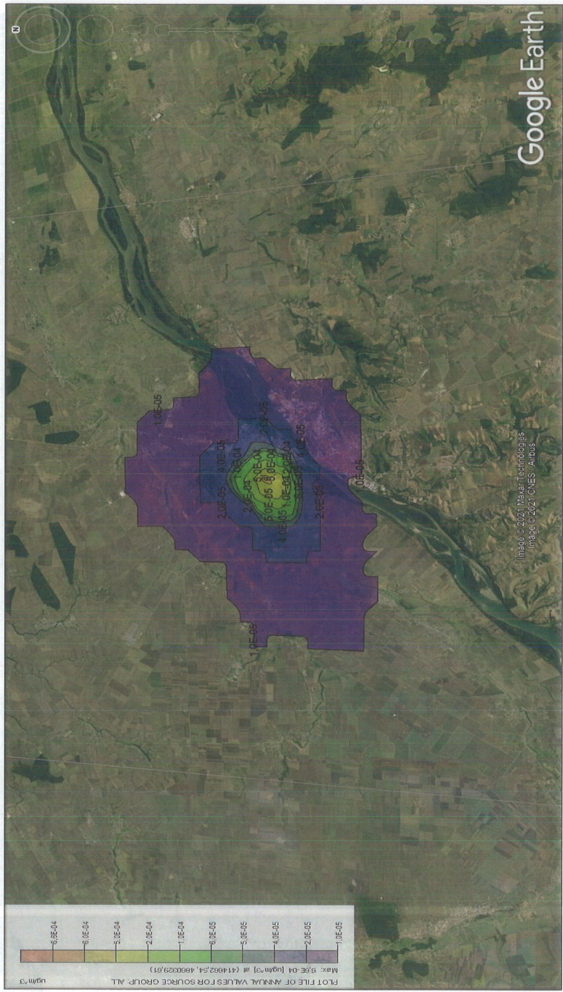
Figure 56 - TSP dispersion modelling - averaging period 1 year
