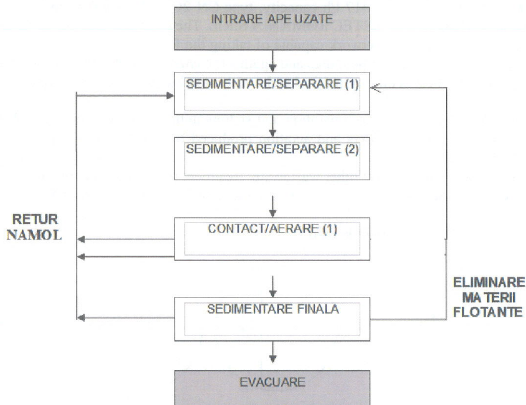
Figure 14 - Diagram of processes of wastewater treatment plant
