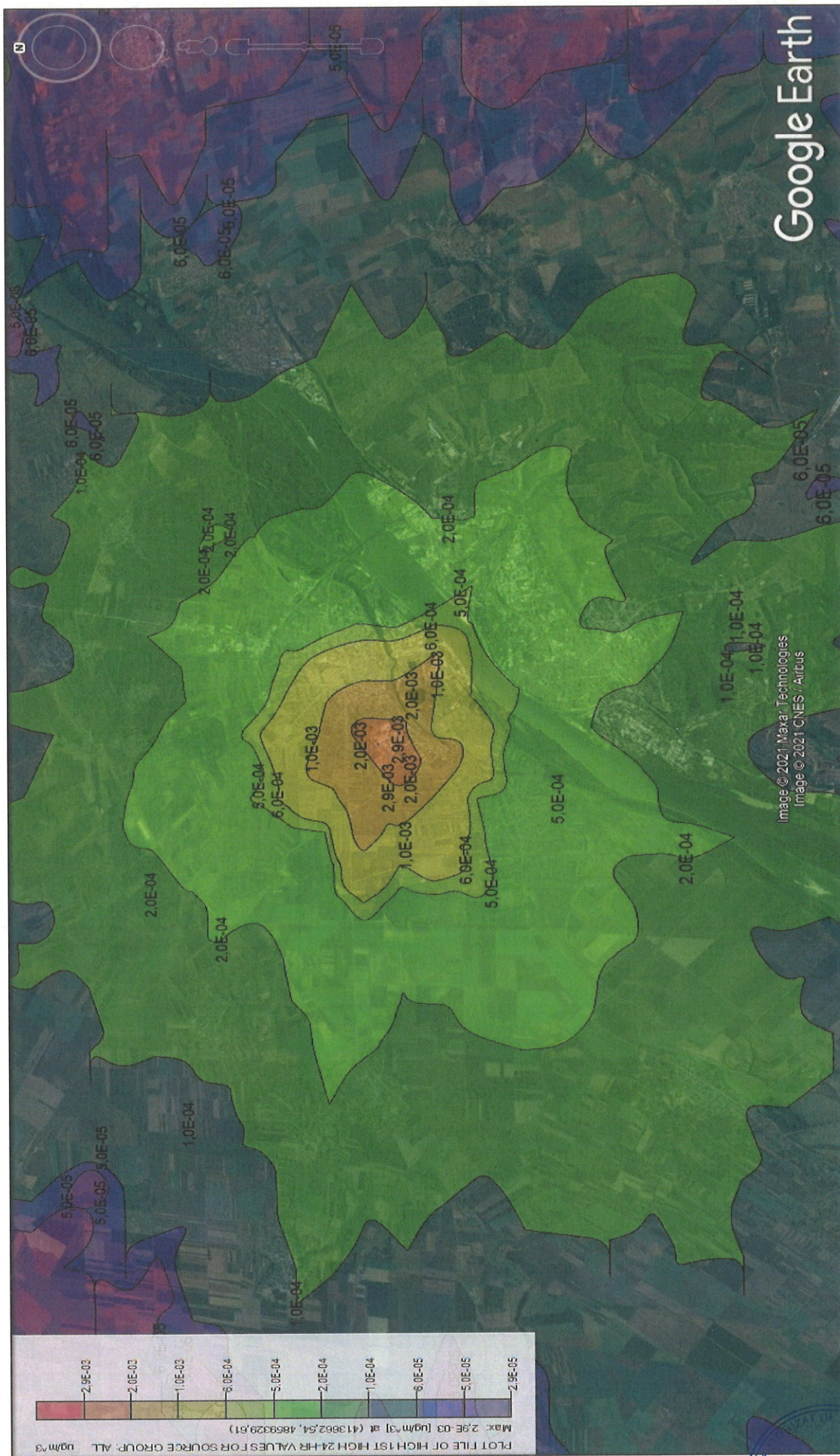
Figure 55 - TSP dispersion modelling - averaging period 1 day (detail)
