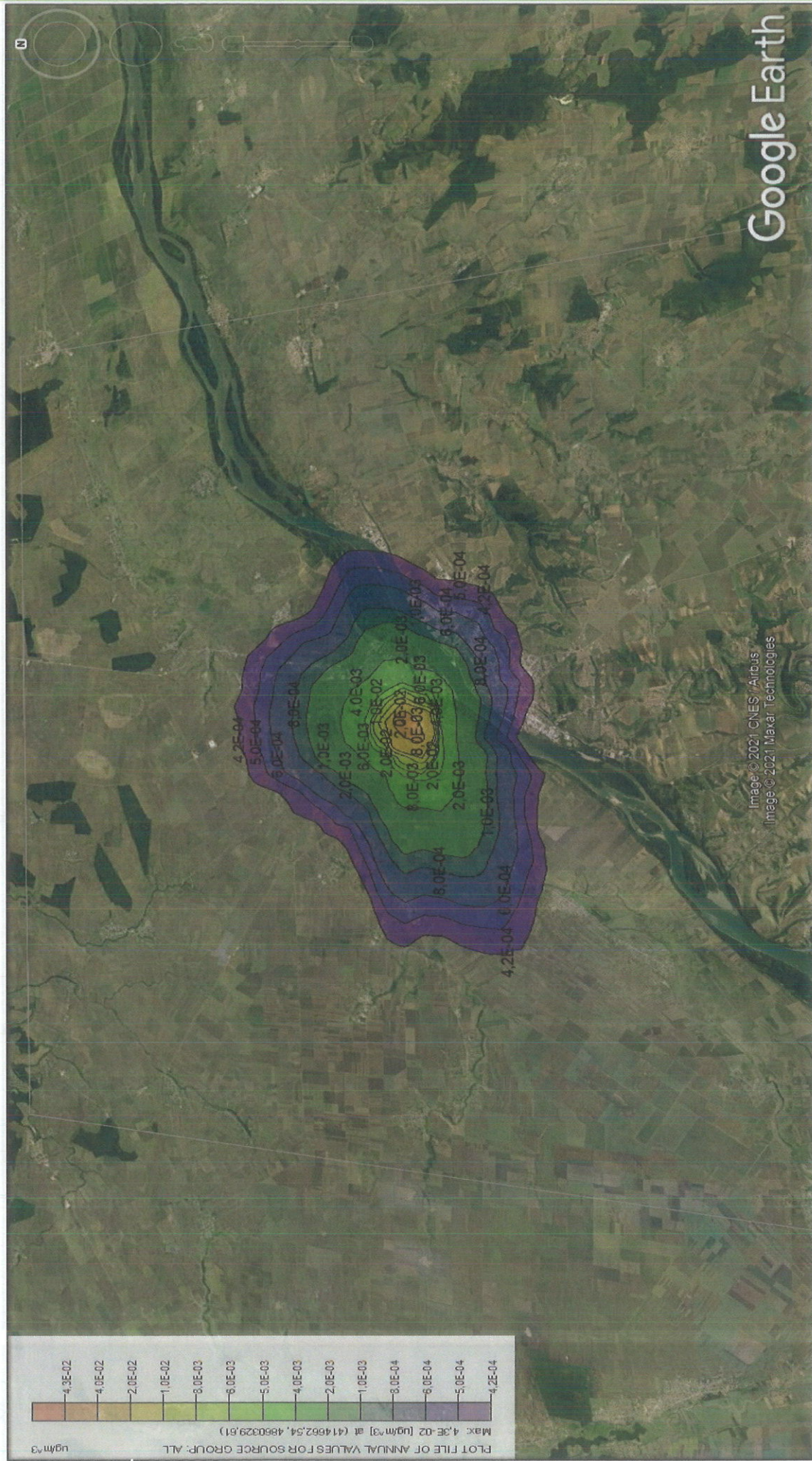
Figure 50 - CO dispersion modelling - averaging period 1 year
