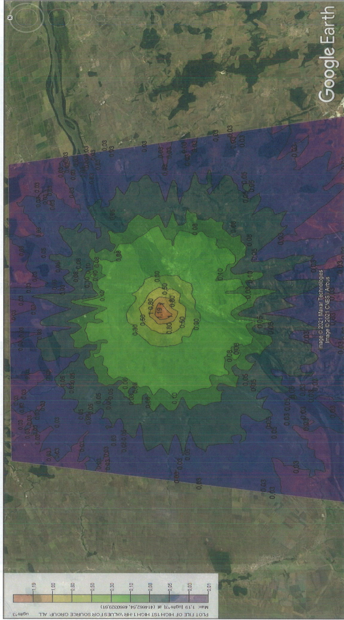
Figure 40 - NO x dispersion modelling - averaging period 1 h
