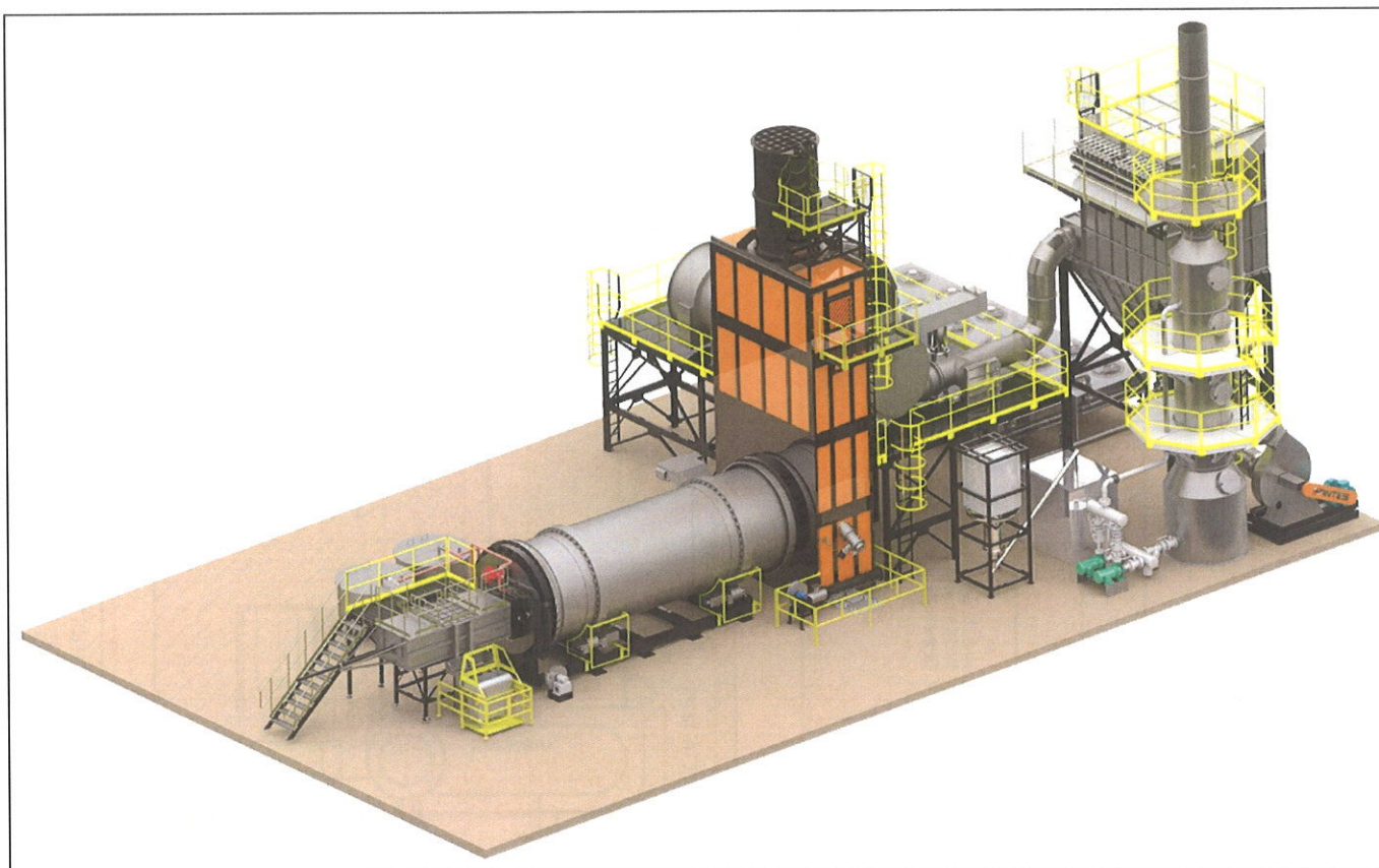
Figure 5 - Incinerator overview
