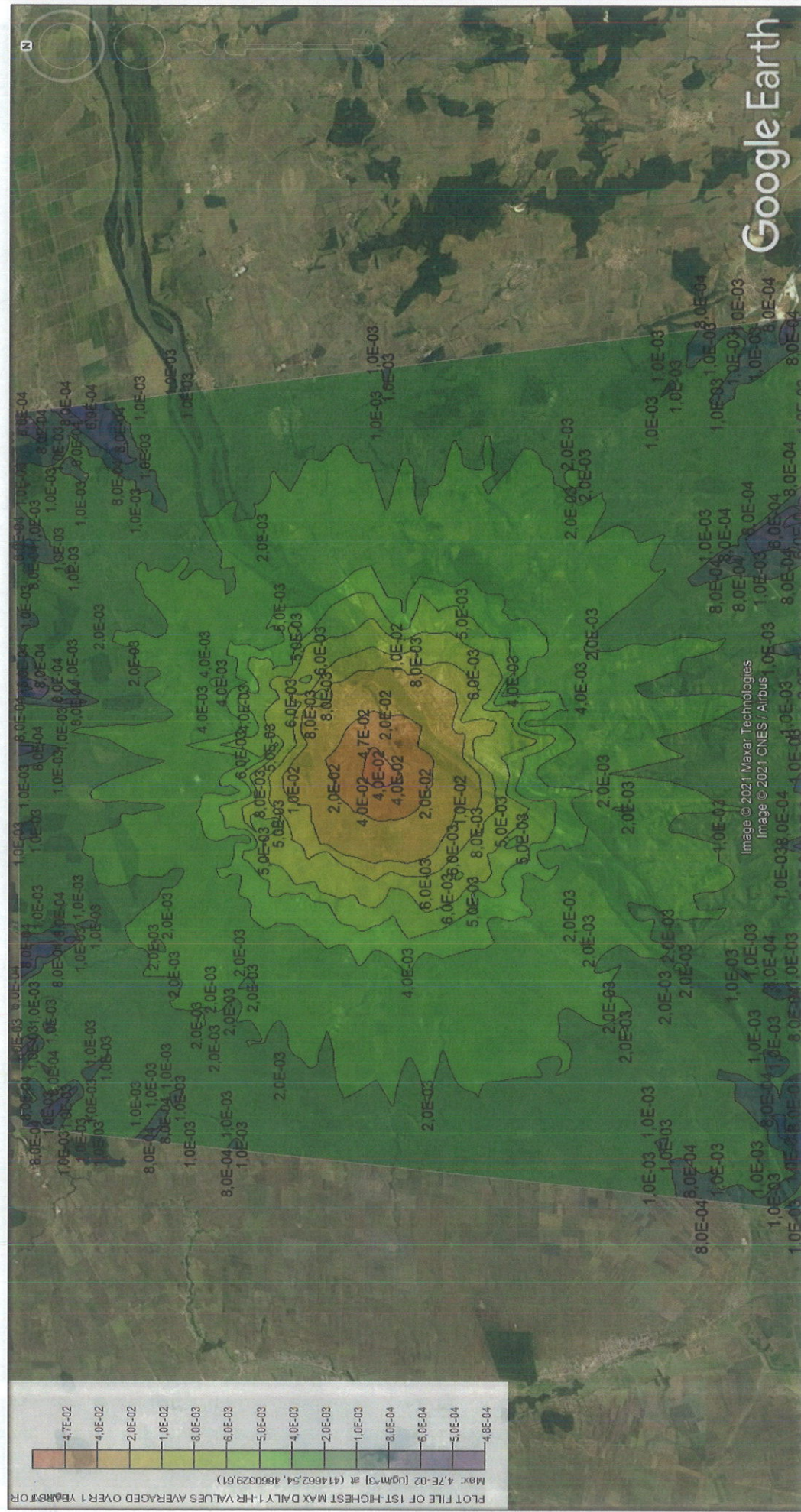
Figure 58 - SO 2 dispersion modelling - 1h averaging period
