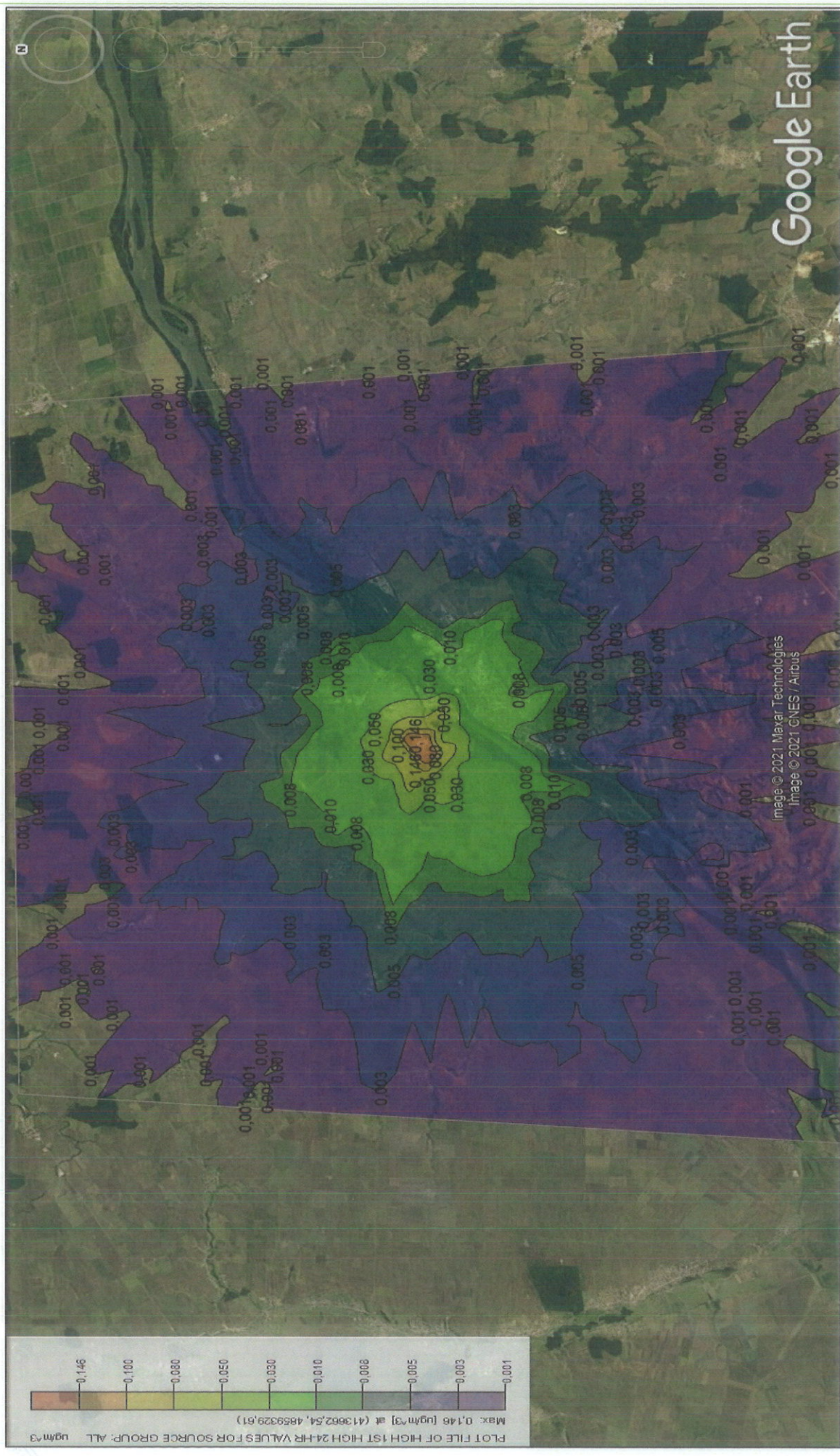
Figure 42 - NOx dispersion modelling - 24 h averaging period
