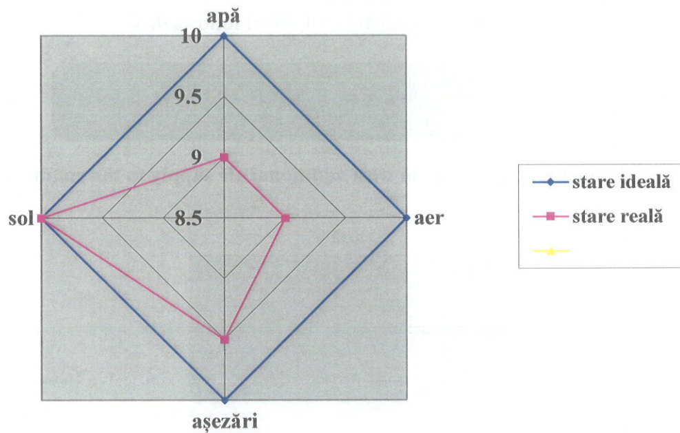
Figure 34 - IPG diagram at the border with Bulgaria
