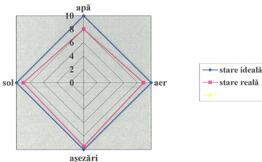
Figure 33 - IPG diagram with additional air supply to the combustion system
