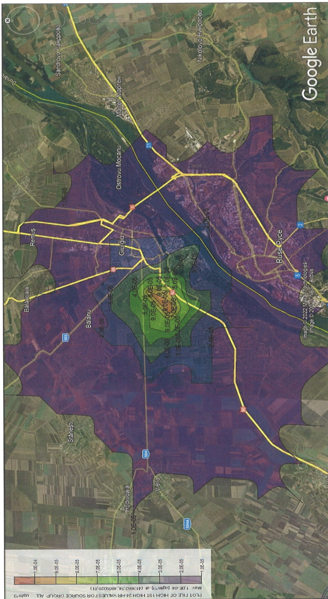
Figure 81 - Modelling of dioxin and furan concentration dispersion in immisions - 24 h averaging period
