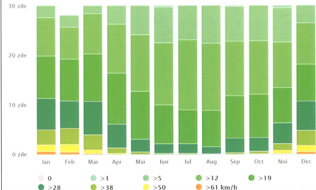
Figure 20 - Modelling annual wind speed variation
