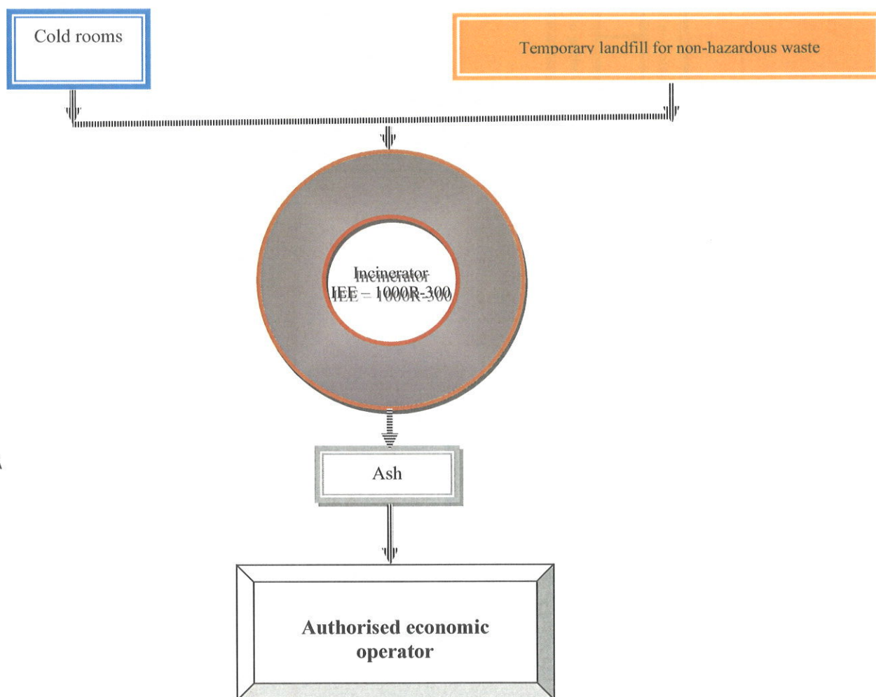
Figure 10 - Non-hazardous waste stream
