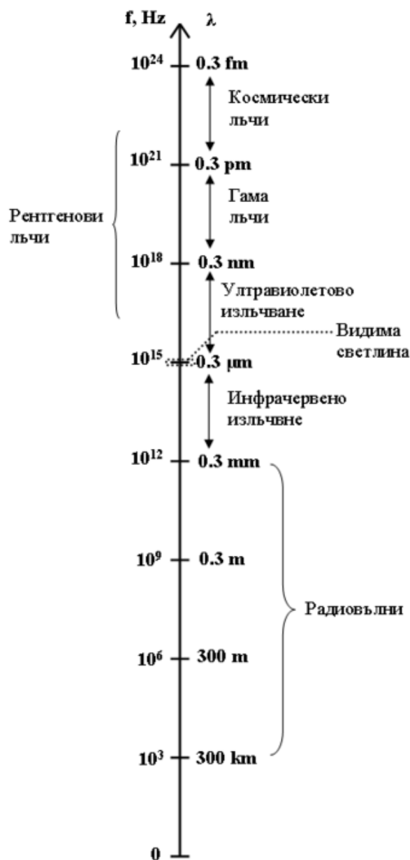
Fig 3.9.2-1 Electromagnetic spectrum
