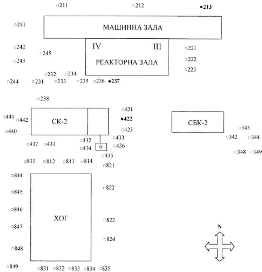
Fig. 3.2.3.4-1 Boreholes around Units 3 and 4, AB-2 and SFSF
