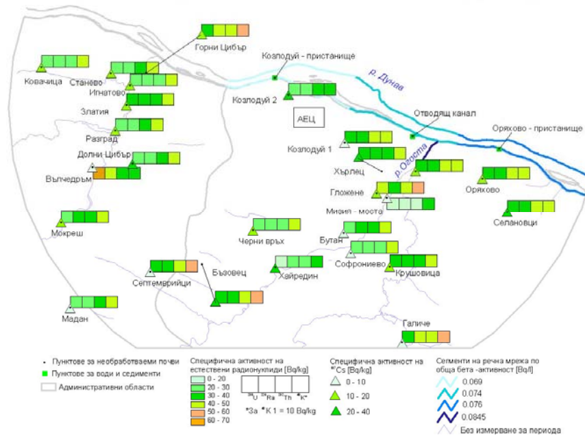
Fig. 3.2.2.1-6 Radiation status of the environment in the KNPP 30-km area for 2009, Source: ExEA
