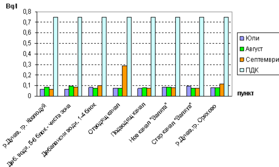
Fig. 3.2.2.1-7 Total tritium activity [Bq/l] in debalanced waters of KNPP and the Danube River
