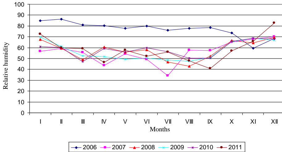
Fig. 3.7-3 Monthly allocation of the values of relative air humidity in the region of KNPP within the period 2006 - 2011
