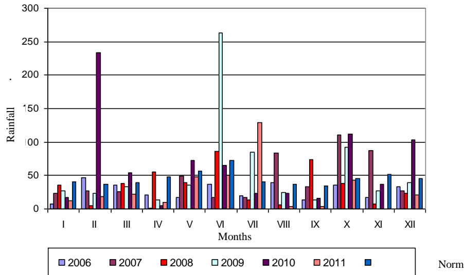
Fig. 3.7-2 Allocation of the month rainfalls in the region of KNPP within 2006– 2011
