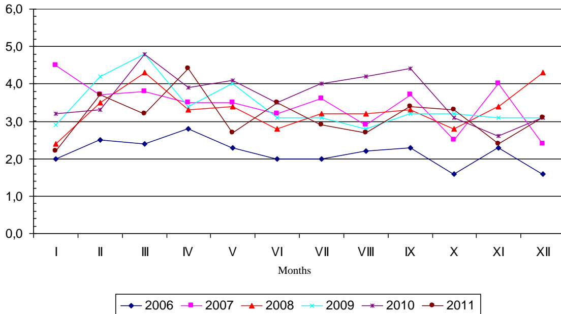
Fig. 3.7-4 Allocation of the average month velocities of the wind in the region of KNPP within the period 2006 – 2011
