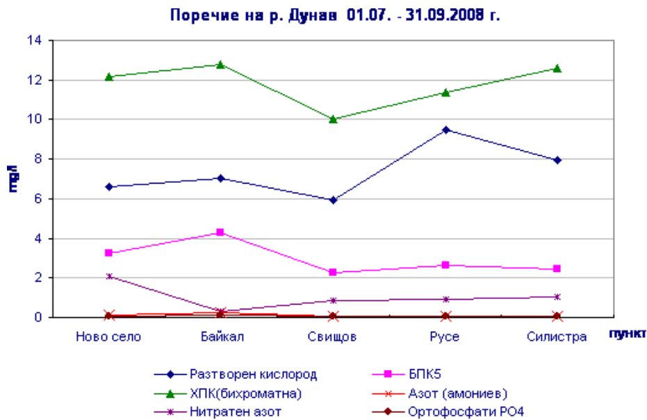
Fig. 3.2.2.2-2 Values of measured indicators at some stations along the Danube River
